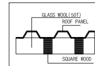
2. SIDE DETAIL
